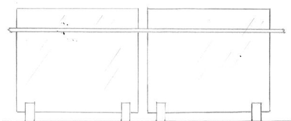
4 – Spigot Mounted (Deck/Paving) Reduced handrail Height
